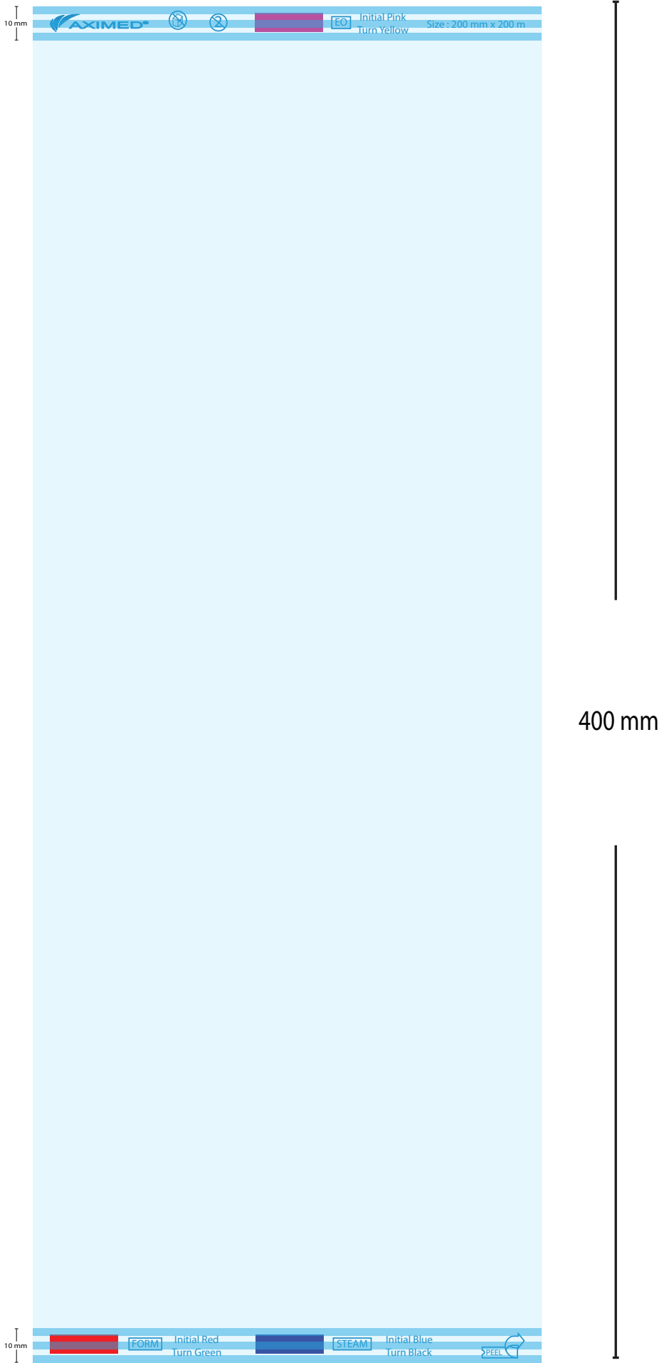
Design Pouch Flat 400 mm
